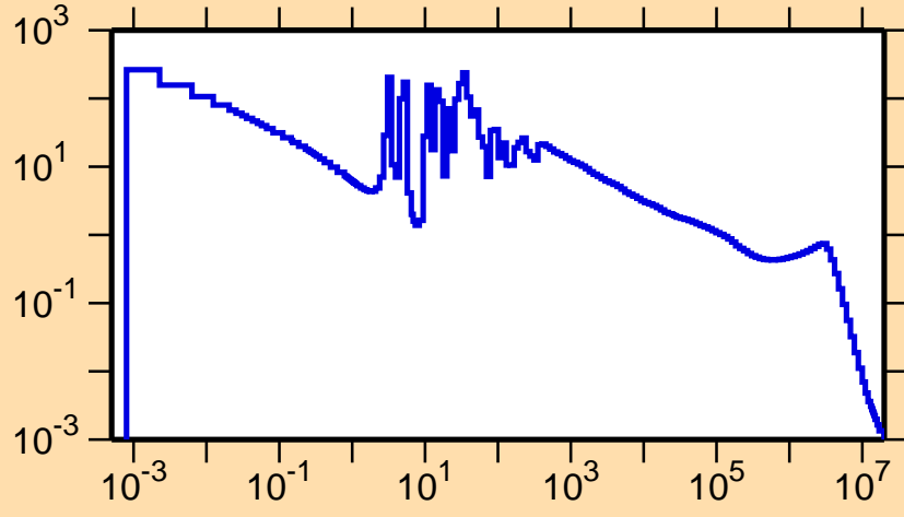
\sigma vs. E for ^{125}\text{Cs}(n,\gamma)
