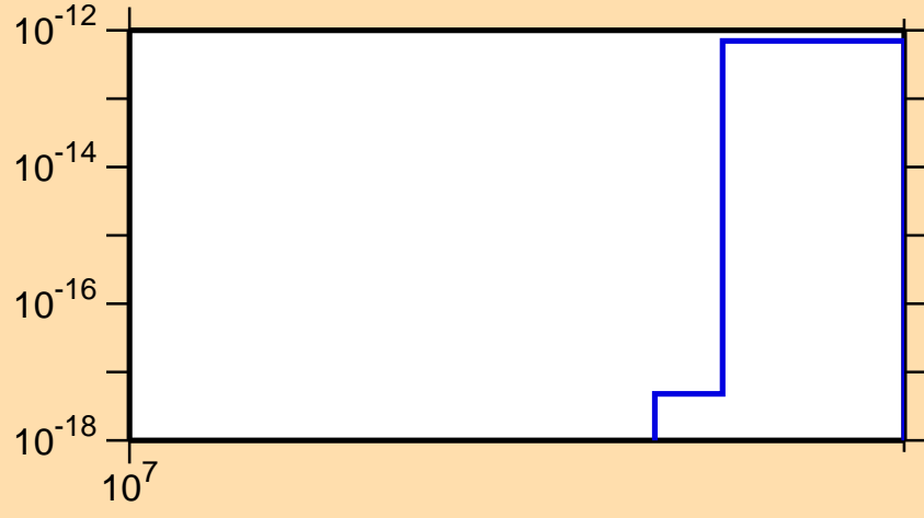
\sigma vs. E for ^{125}\text{Cs}(n,\text{pt})
