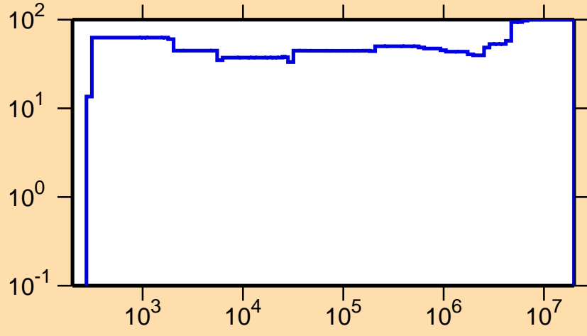
\Delta\sigma/\sigma vs. E for ^{125}\text{Cs}(n,\gamma)
