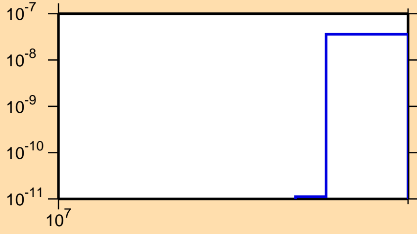
\sigma vs. E for ^{125}\text{Cs}(n,nt)
