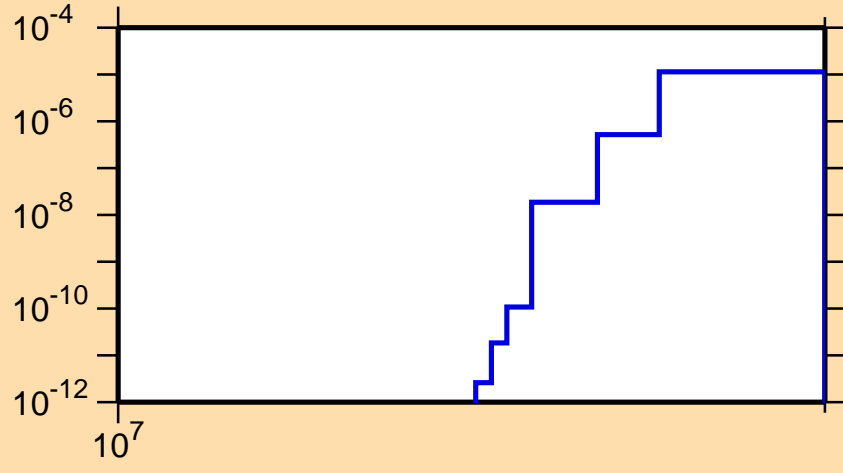
\sigma vs. E for ^{125}\text{Cs}(n,\text{nd})
