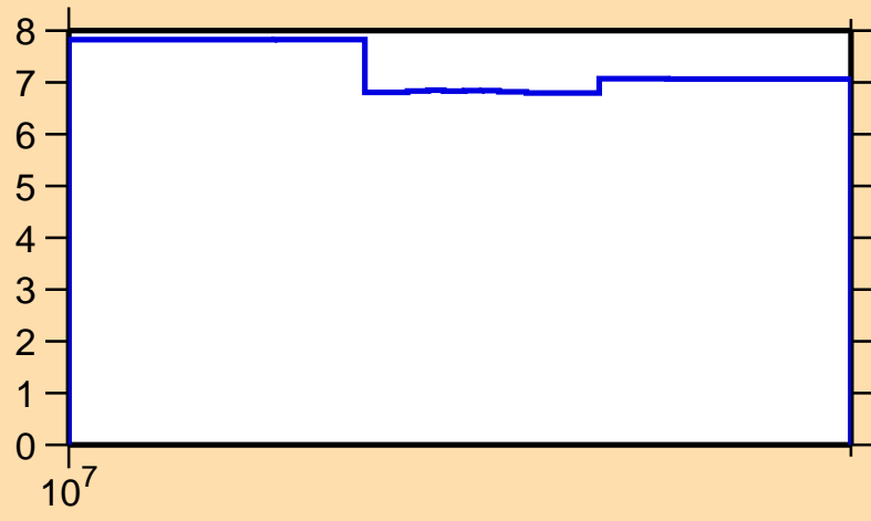
\Delta\sigma/\sigma vs. E for ^{125}\text{Cs}(n,\text{nonel.})
