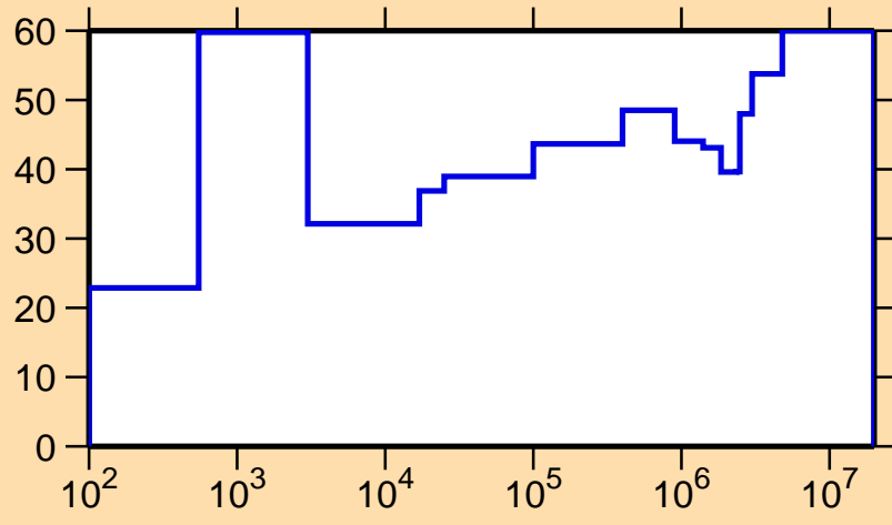
\Delta\sigma/\sigma vs. E for ^{125}\text{Cs}(n,\gamma)
