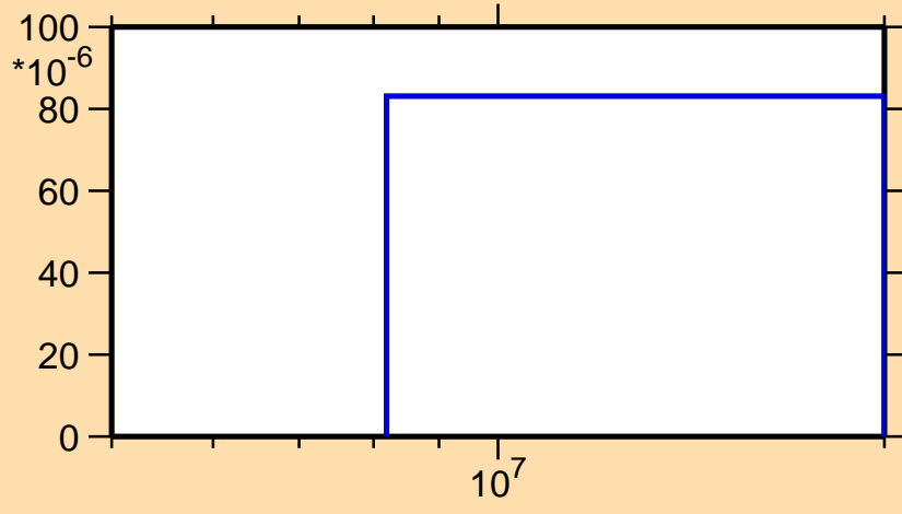
\sigma vs. E for ^{125}\text{Cs}(n,t)
