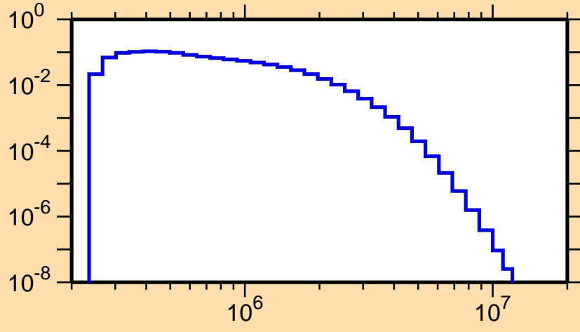
\sigma vs. E for ^{126}\text{Cs}(n,n_2)
