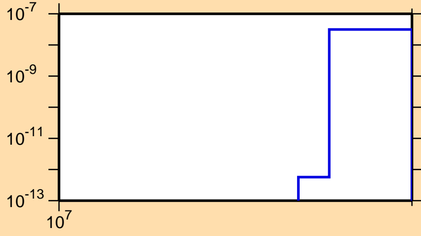
\sigma vs. E for ^{126}\text{Cs}(n,nt)
