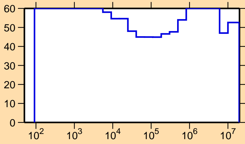
\Delta\sigma/\sigma vs. E for ^{126}\text{Cs}(n,\gamma)
