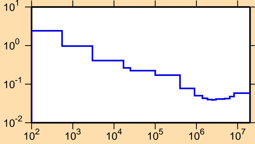
\sigma vs. E for ^{126}\text{Cs}(n,p)
