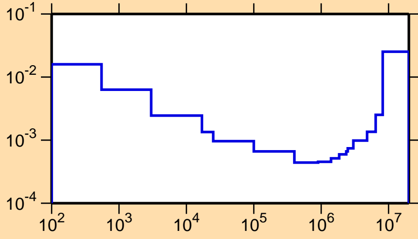
\sigma vs. E for ^{126}\text{Cs}(n,\alpha)
