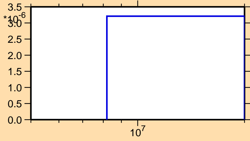
\sigma vs. E for ^{126}\text{Cs}(n,nd)
