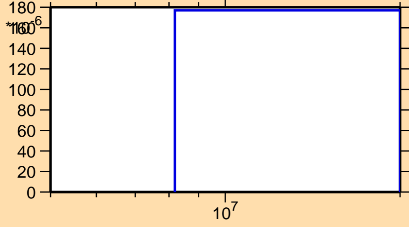
\sigma vs. E for ^{126}\text{Cs}(n,2np)
