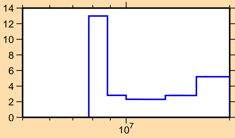
\Delta\sigma/\sigma vs. E for ^{128}\text{Cs}(n,2n)
