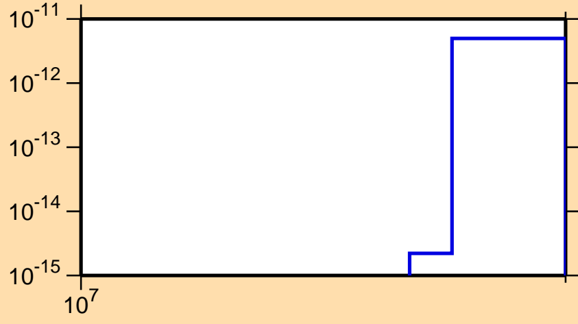
\sigma vs. E for ^{128}\text{Cs}(n,pt)
