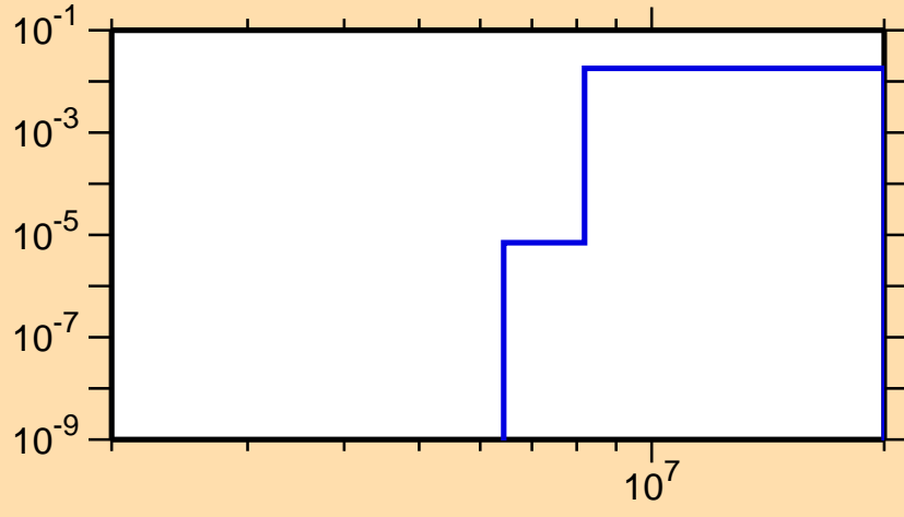
\sigma vs. E for ^{128}\text{Cs}(n,np)
