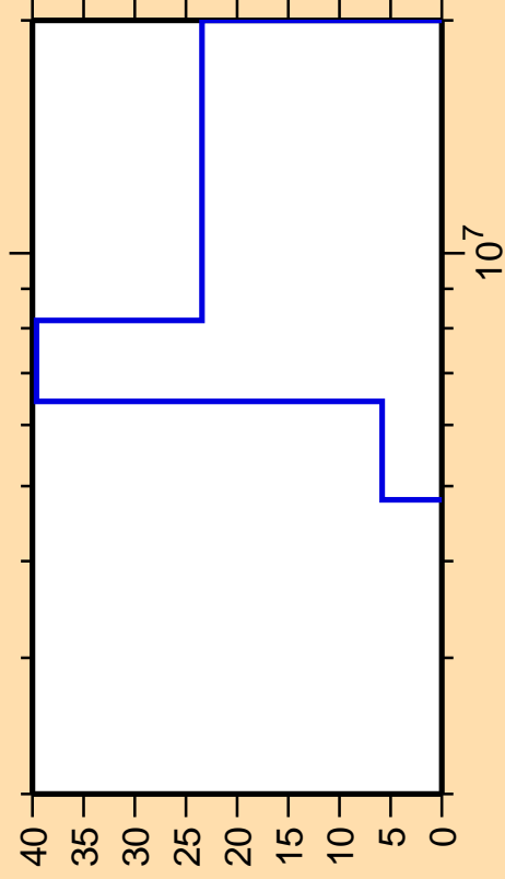
\Delta\sigma/\sigma vs. E for ^{128}\text{Cs}(n,np)
