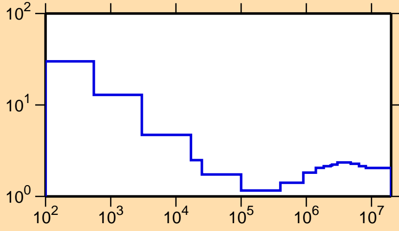
\sigma vs. E for ^{128}\text{Cs}(n,\text{nonel.})
