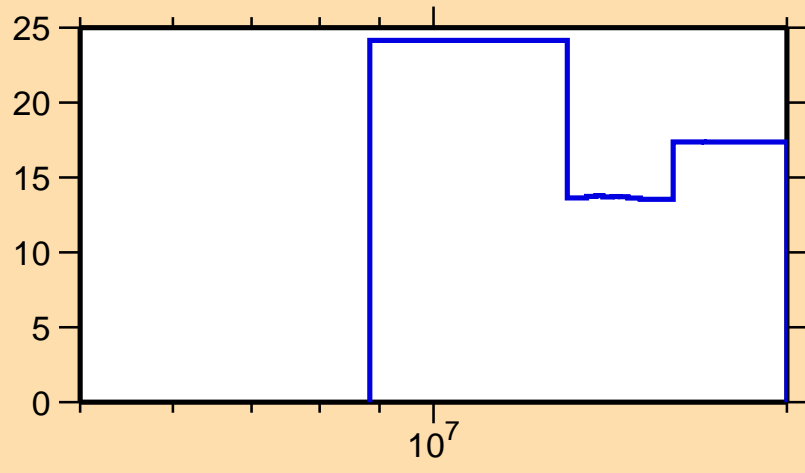
\Delta\sigma/\sigma vs. E for ^{129}\text{Cs}(n,2n)
