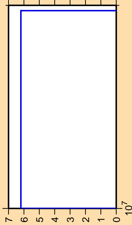
\Delta\sigma/\sigma vs. E for ^{129}\text{Cs}(\text{mt117})
