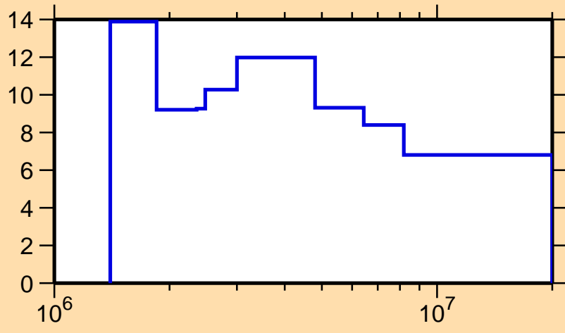
\Delta\sigma/\sigma vs. E for ^{129}\text{Cs}(n,\text{nonel.})
