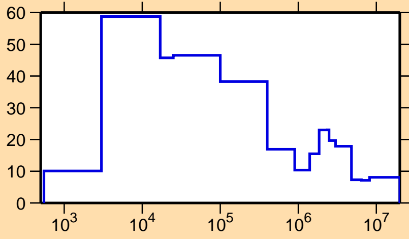
\Delta\sigma/\sigma vs. E for ^{129}\text{Cs}(n,\text{el.})
