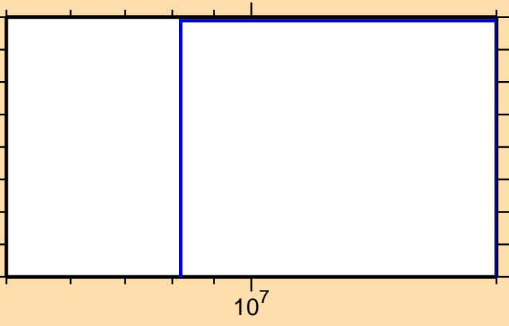
\sigma vs. E for ^{129}\text{Cs}(\text{mt117})
