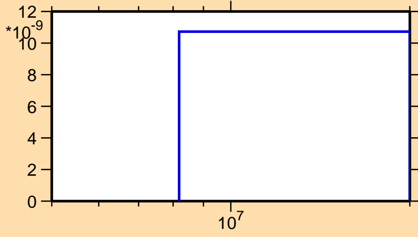
\sigma vs. E for ^{129}\text{Cs}(n,p\alpha)
