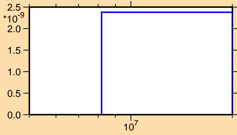
\sigma vs. E for ^{129}\text{Cs}(n,\text{He}3)
