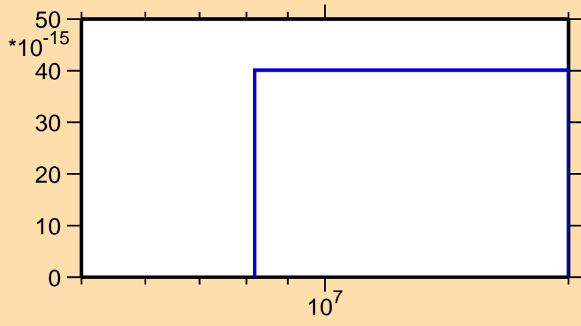
\sigma vs. E for ^{129}\text{Cs}(n,\text{pd})
