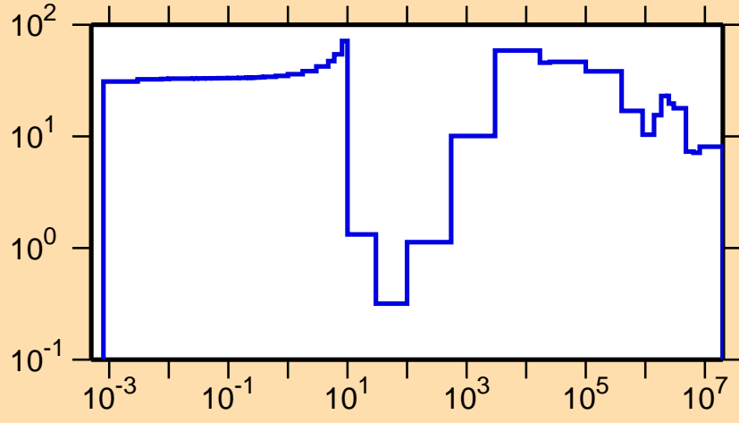
\Delta\sigma/\sigma vs. E for ^{129}\text{Cs}(n,\text{el.})
