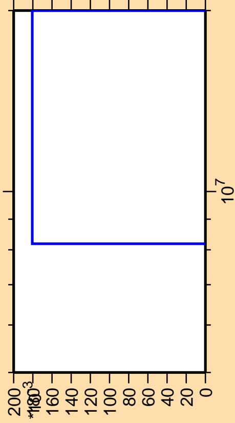
\Delta\sigma/\sigma vs. E for ^{129}\text{Cs}(n,\text{pd})
