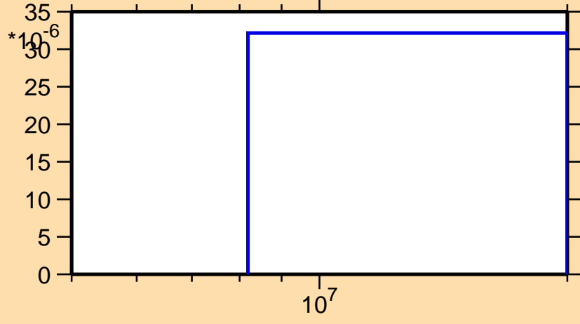
\sigma vs. E for ^{129}\text{Cs}(n,3n)
