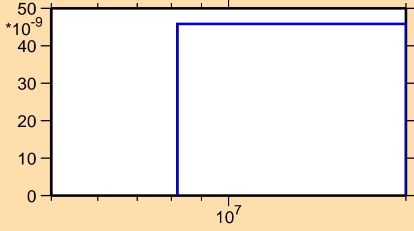
\sigma vs. E for ^{129}\text{Cs}(n,nd)
