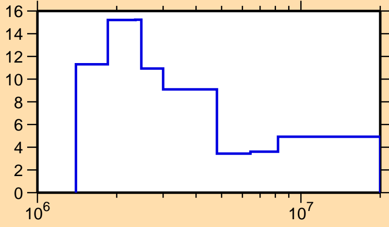
\Delta\sigma/\sigma vs. E for ^{129}\text{Cs}(n,\text{tot.})
