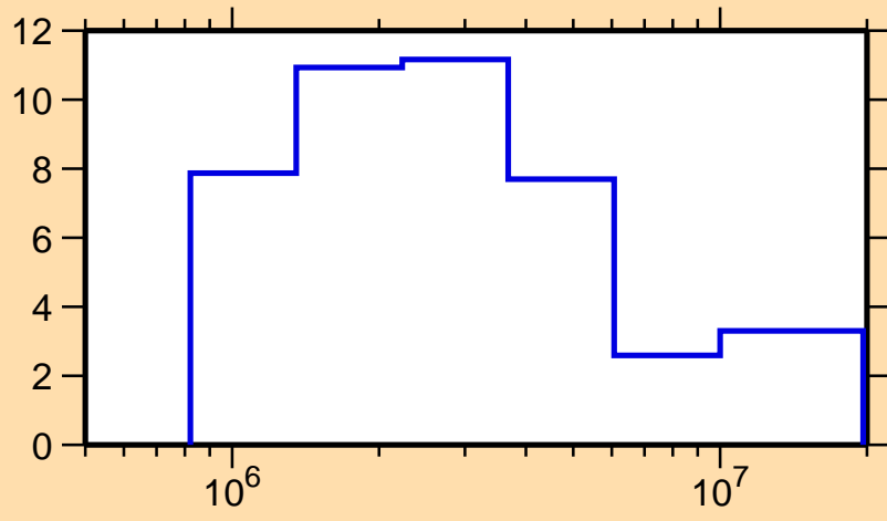
\Delta\sigma/\sigma vs. E for ^{130}\text{Cs}(n,\text{tot.})
