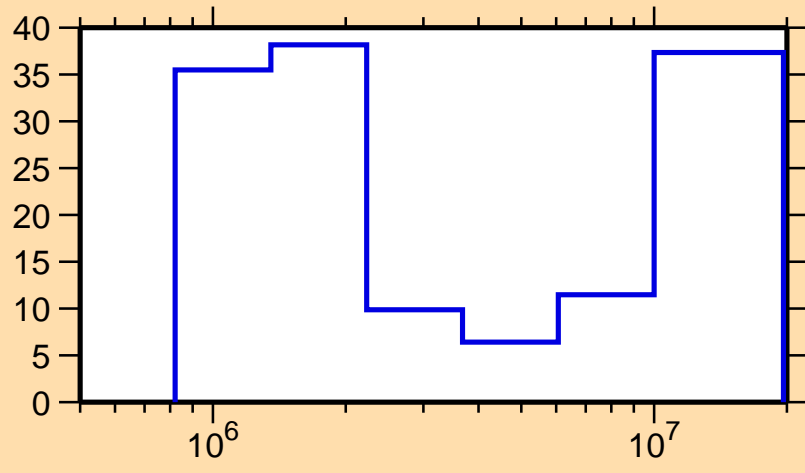
\Delta\sigma/\sigma vs. E for ^{130}\text{Cs}(n,n\text{cont.})
