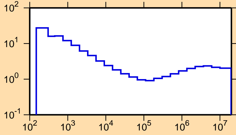
\sigma vs. E for ^{130}\text{Cs}(n,\text{nonel.})
