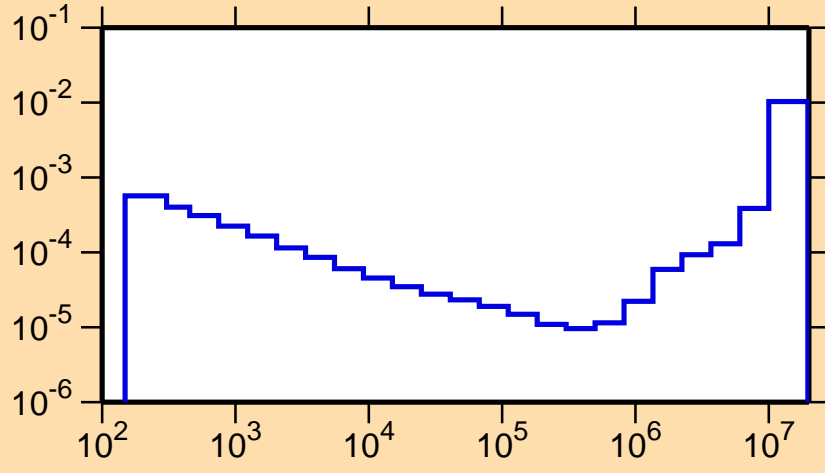
\sigma vs. E for ^{130}\text{Cs}(n,\alpha)
