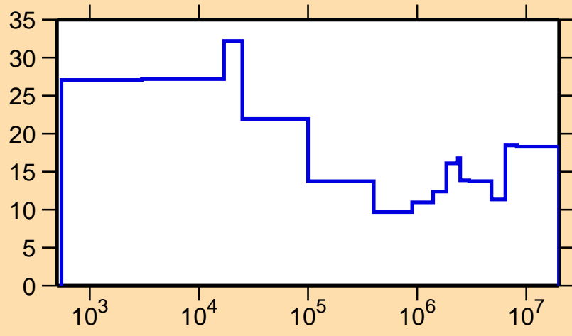
\Delta\sigma/\sigma vs. E for ^{130}\text{Cs}(n,n_1)
