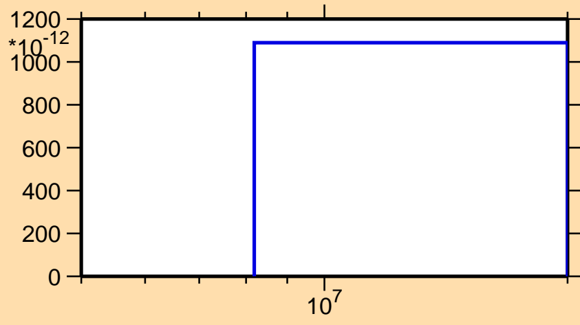
\sigma vs. E for ^{130}\text{Cs}(n,nt)
