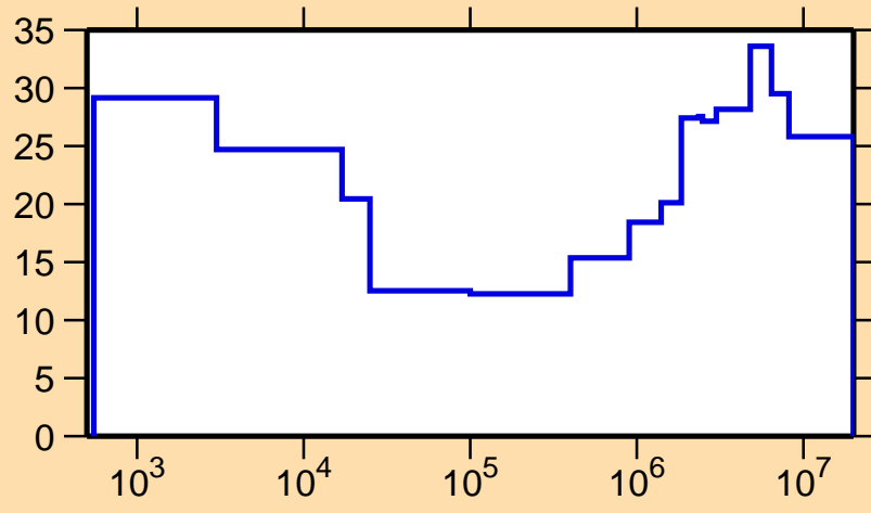
\Delta\sigma/\sigma vs. E for ^{130}\text{Cs}(n,\gamma)
