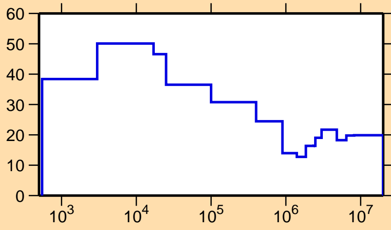
\Delta\sigma/\sigma vs. E for ^{130}\text{Cs}(n,p)
