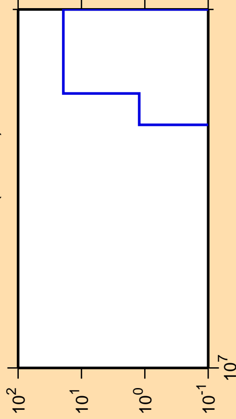
\Delta\sigma/\sigma vs. E for ^{131}\text{Cs}(\text{mt117})
