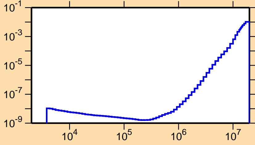
\sigma vs. E for ^{131}\text{Cs}(n,\alpha)
