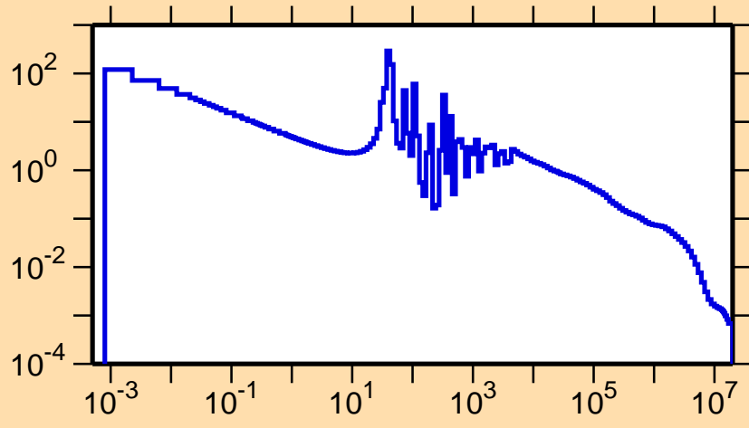
\sigma vs. E for ^{131}\text{Cs}(n,\gamma)
