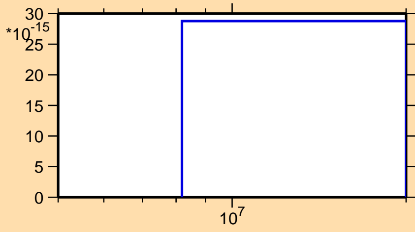
\sigma vs. E for ^{131}\text{Cs}(\text{mt117})
