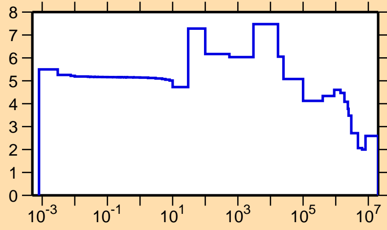
\sigma vs. E for ^{131}\text{Cs}(n,\text{el.})
