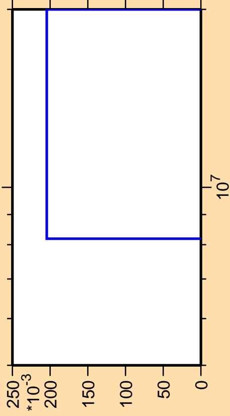
\Delta\sigma/\sigma vs. E for ^{131}\text{Cs}(\text{mt117})
