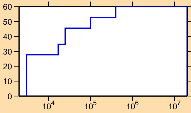
\Delta\sigma/\sigma vs. E for ^{131}\text{Cs}(n,\gamma)
