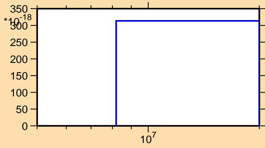
\sigma vs. E for ^{131}\text{Cs}(n,\text{pd})
