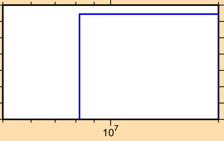
\sigma vs. E for ^{131}\text{Cs}(n,\text{nd})
