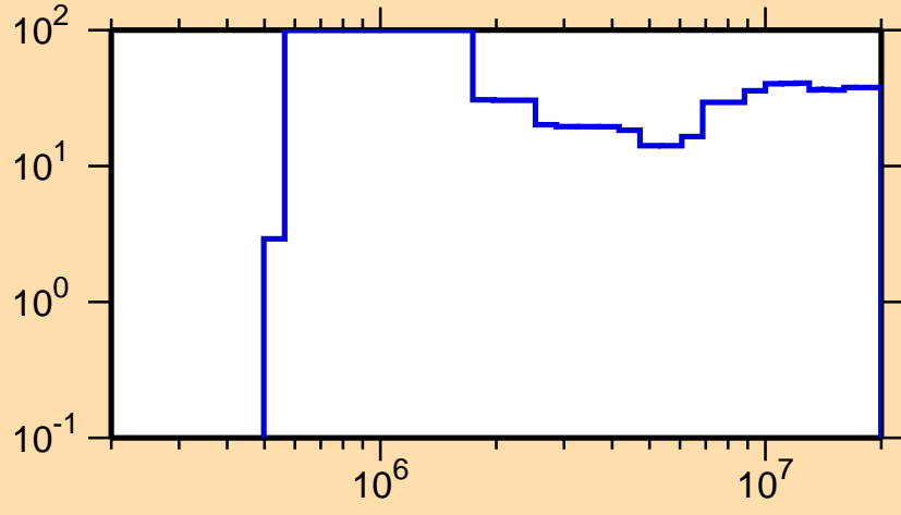
\Delta\sigma/\sigma vs. E for ^{132}\text{Cs}(n,n\text{cont.})
