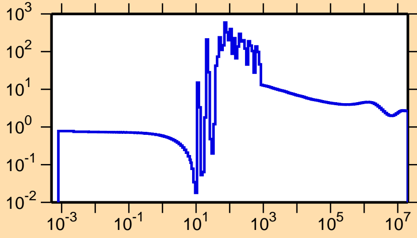
\sigma vs. E for ^{132}\text{Cs}(n,\text{el.})
