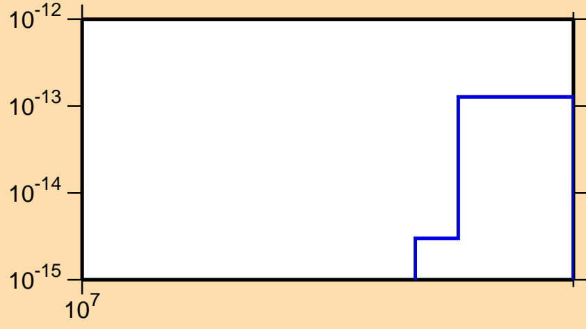
\sigma vs. E for ^{132}\text{Cs}(\text{mt117})
