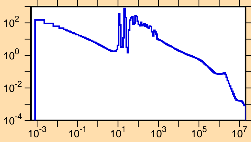
\sigma vs. E for ^{132}\text{Cs}(n,\gamma)
