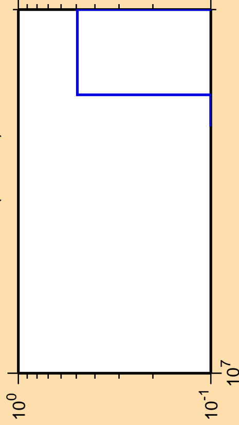
\Delta\sigma/\sigma vs. E for ^{132}\text{Cs}(\text{mt117})
