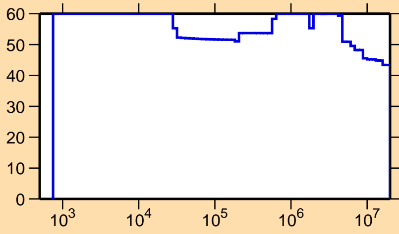
\Delta\sigma/\sigma vs. E for ^{132}\text{Cs}(n,p)
