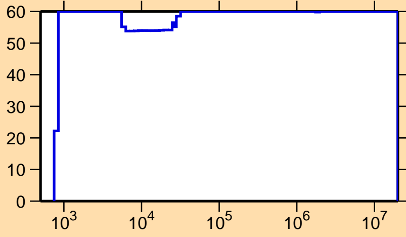
\Delta\sigma/\sigma vs. E for ^{132}\text{Cs}(n,\gamma)
