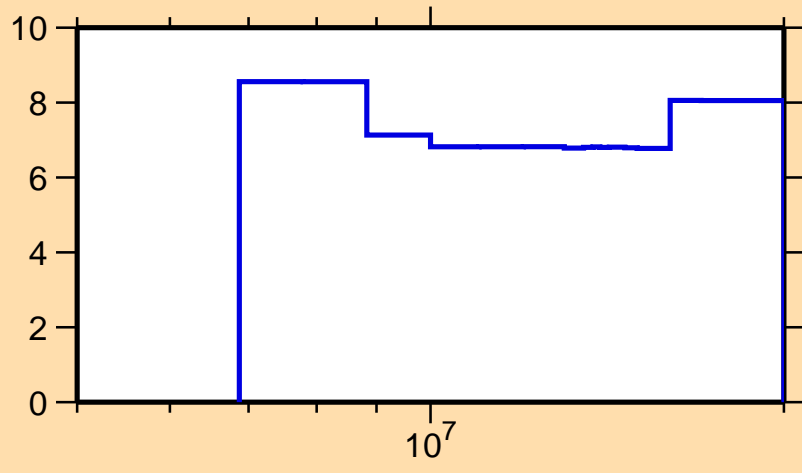
\Delta\sigma/\sigma vs. E for ^{132}\text{Cs}(n,\text{nonel.})
