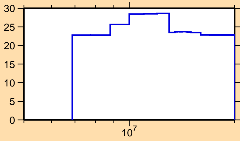
\Delta\sigma/\sigma vs. E for ^{132}\text{Cs}(n,\text{inel.})
