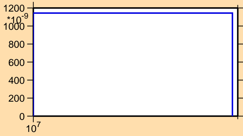
\sigma vs. E for ^{132}\text{Cs}(n,\text{nd})
