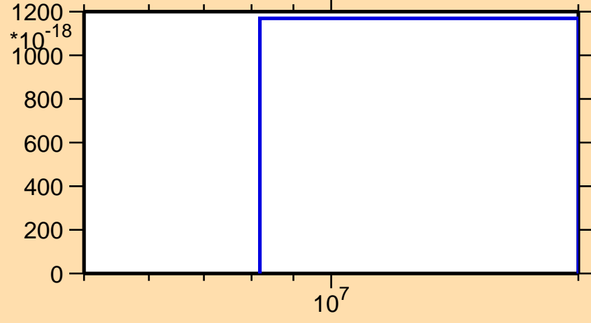
\sigma vs. E for ^{132}\text{Cs}(\text{mt117})
