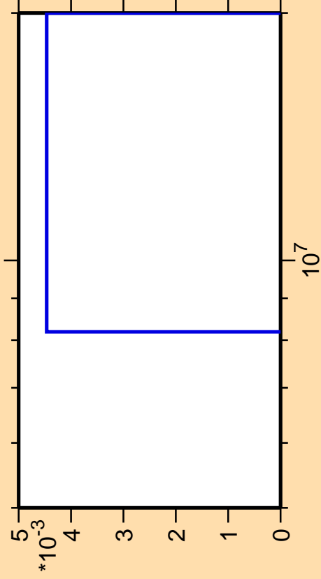
\Delta\sigma/\sigma vs. E for ^{132}\text{Cs}(\text{mt117})
