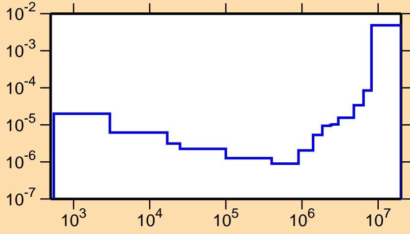
\sigma vs. E for ^{132}\text{Cs}(n,\alpha)
