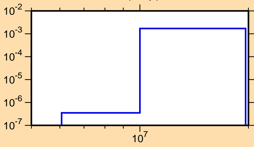
\sigma vs. E for ^{133}\text{Cs}(n,np)
