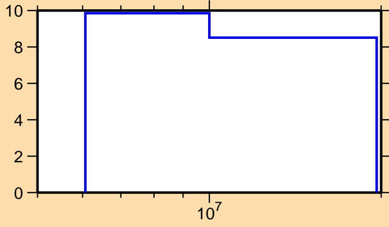
\Delta\sigma/\sigma vs. E for ^{133}\text{Cs}(n,2n)
