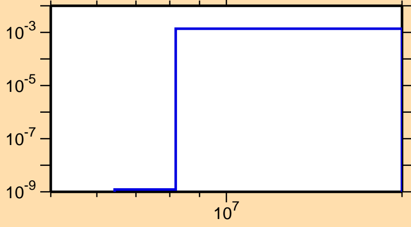
\sigma vs. E for ^{133}\text{Cs}(n,np)
