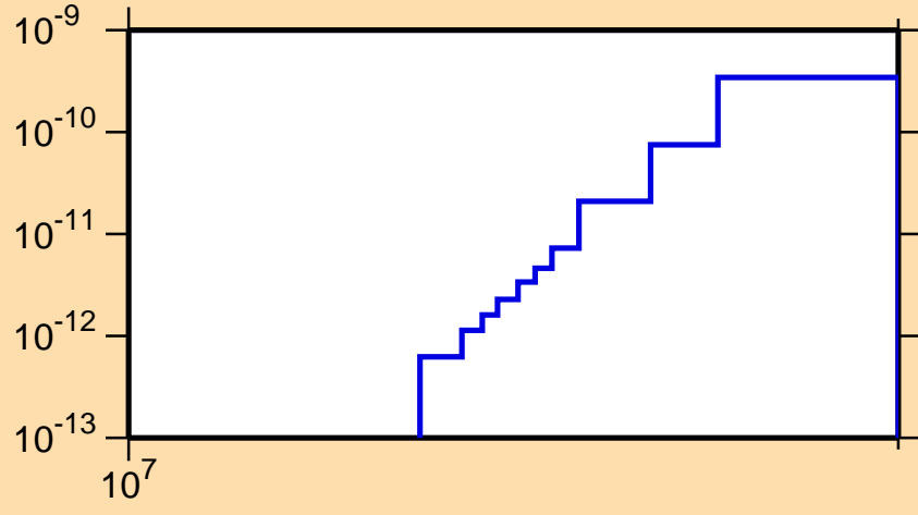
\sigma vs. E for ^{134}\text{Cs}(n,p\alpha)
