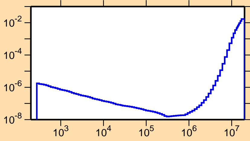
\sigma vs. E for ^{134}\text{Cs}(n,\alpha)
