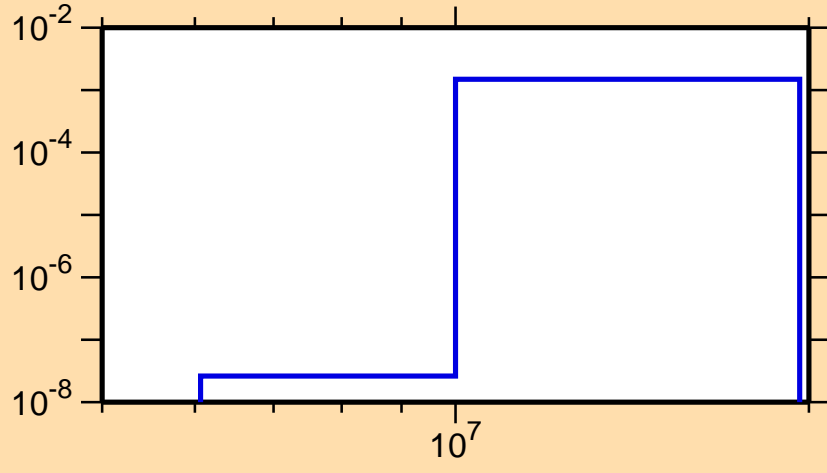
\sigma vs. E for ^{135}\text{Cs}(n,d)
