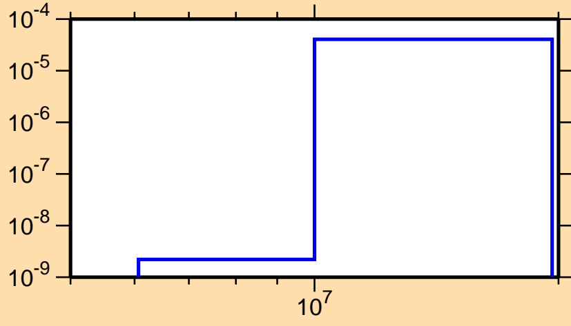
\sigma vs. E for ^{135}\text{Cs}(n,n\alpha)
