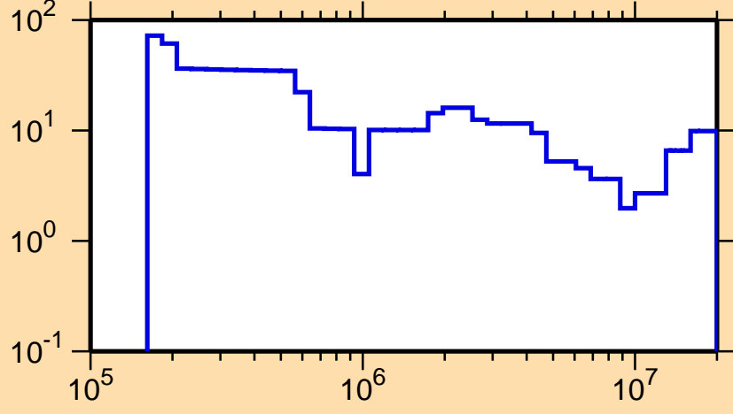
\Delta\sigma/\sigma vs. E for ^{135}\text{Cs}(n, tot.)
