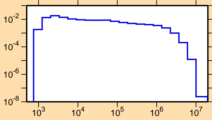
\sigma vs. E for ^{135}\text{Cs}(n,n_1)
