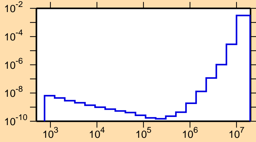
\sigma vs. E for ^{135}\text{Cs}(n,\alpha)
