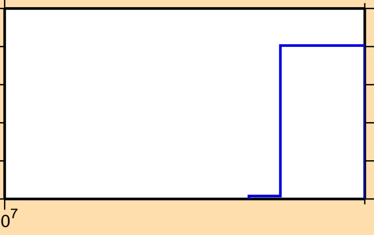
\sigma vs. E for ^{136}\text{Cs}(n,nt)
