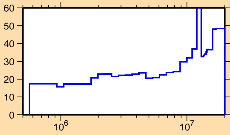
\Delta\sigma/\sigma vs. E for ^{136}\text{Cs}(n,n_1)
