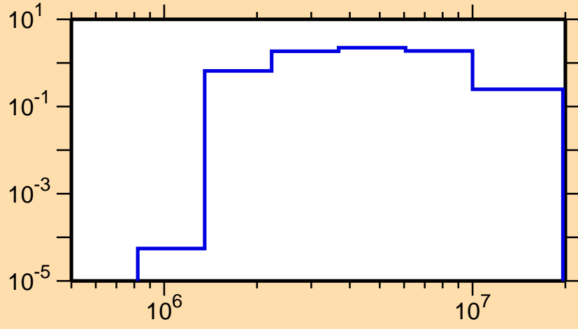
\sigma vs. E for ^{136}\text{Cs}(n,n\text{cont.})
