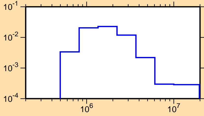
\sigma vs. E for ^{136}\text{Cs}(n,n_3)
