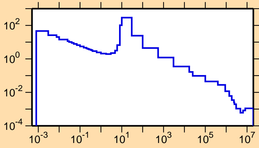
\sigma vs. E for ^{136}\text{Cs}(n,\gamma)
