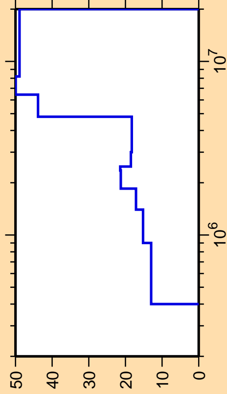
\Delta\sigma/\sigma vs. E for ^{136}\text{Cs}(n,n_4)
