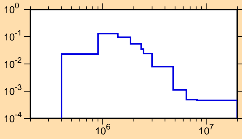
\sigma vs. E for ^{136}\text{Cs}(n,n_4)
