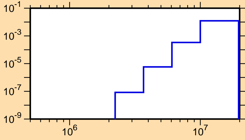
\sigma vs. E for ^{136}\text{Cs}(n,p)
