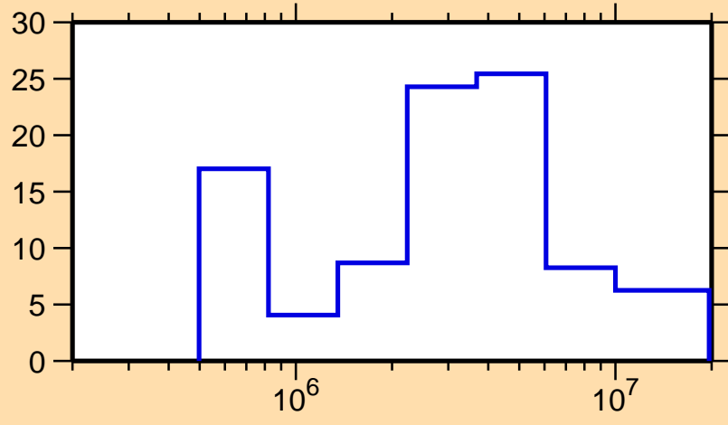
\Delta\sigma/\sigma vs. E for ^{136}\text{Cs}(n,\text{el.})
