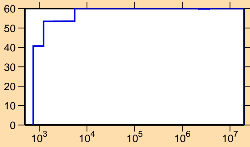
\Delta\sigma/\sigma vs. E for ^{136}\text{Cs}(n,\gamma)
