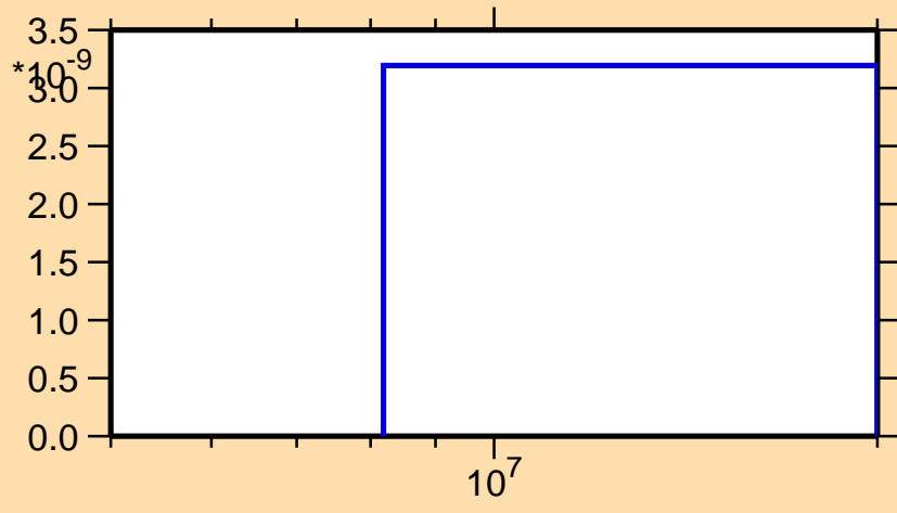
\sigma vs. E for ^{136}\text{Cs}(n,nt)
