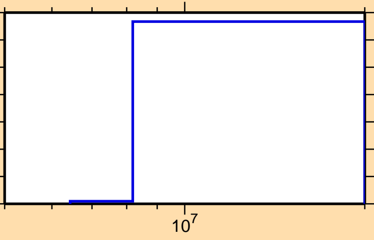
\sigma vs. E for ^{136}\text{Cs}(n,n\alpha)
