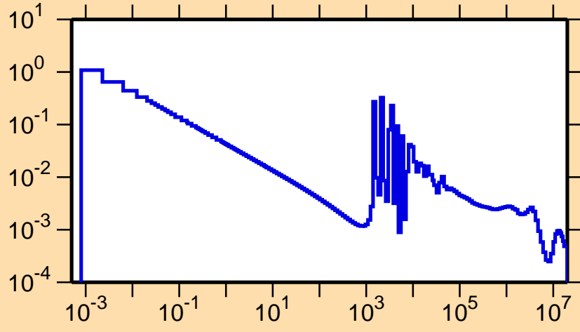
\sigma vs. E for ^{137}\text{Cs}(n,\gamma)
