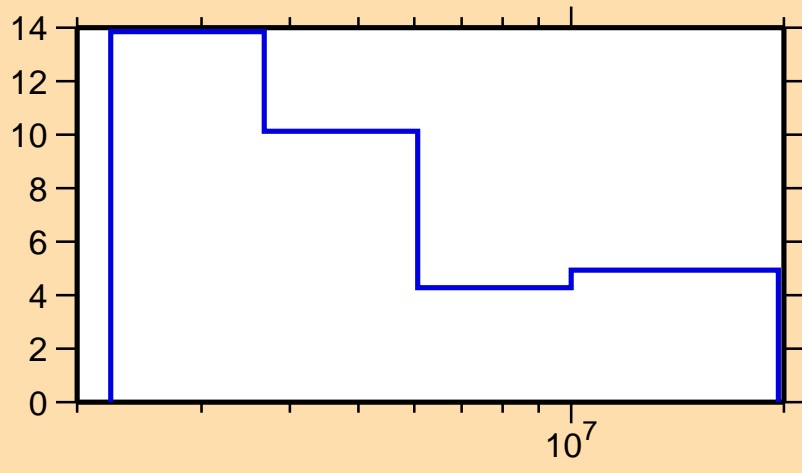
\Delta\sigma/\sigma vs. E for ^{137}\text{Cs}(n, tot.)
