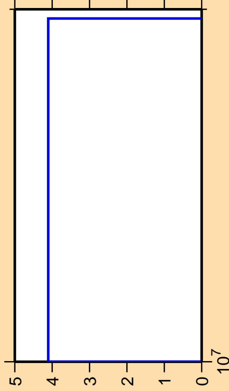
\Delta\sigma/\sigma vs. E for ^{137}\text{Cs}(n,2n\alpha)
