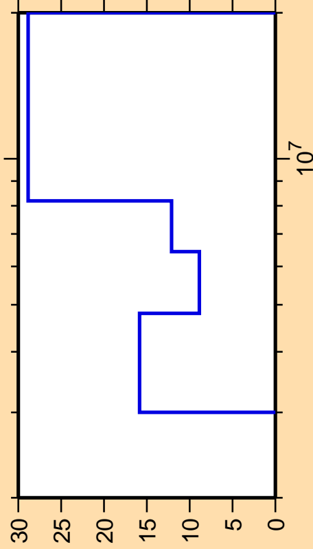
\Delta\sigma/\sigma vs. E for ^{137}\text{Cs}(n, ncont.)
