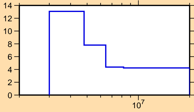
\Delta\sigma/\sigma vs. E for ^{137}\text{Cs}(n, tot.)
