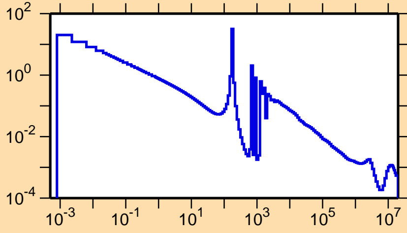
\sigma vs. E for ^{138}\text{Cs}(n,\gamma)
