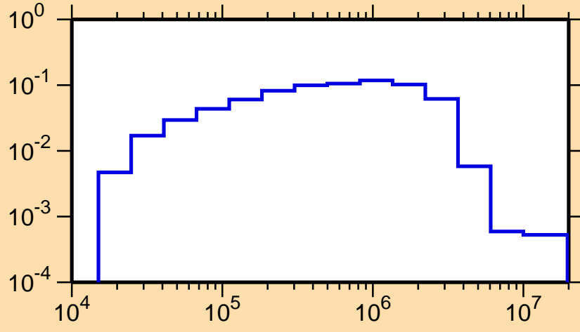
\sigma vs. E for ^{138}\text{Cs}(n,n_2)
