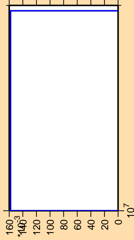
\Delta\sigma/\sigma vs. E for ^{138}\text{Cs}(n,\text{He}3)
