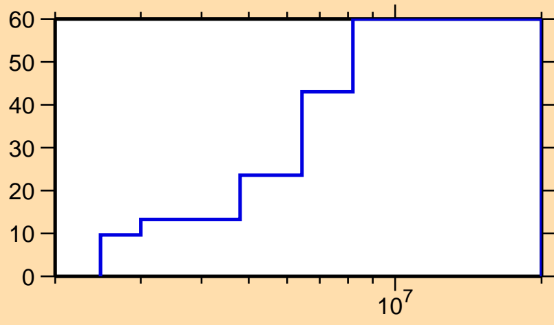
\Delta\sigma/\sigma vs. E for ^{138}\text{Cs}(n,n\text{cont.})
