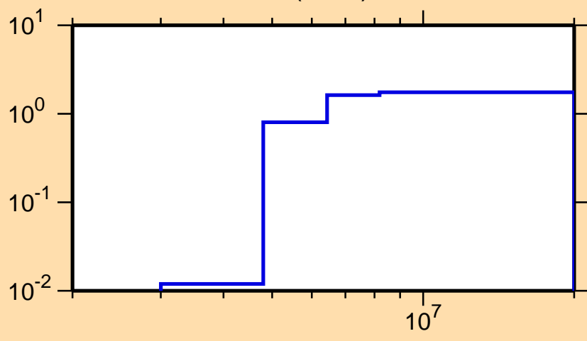
\sigma vs. E for ^{138}\text{Cs}(n,2n)
