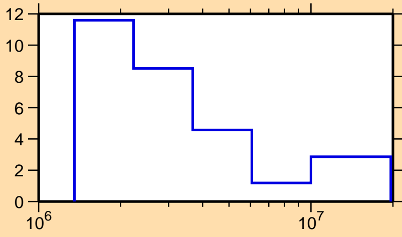
\Delta\sigma/\sigma vs. E for ^{138}\text{Cs}(n, tot.)
