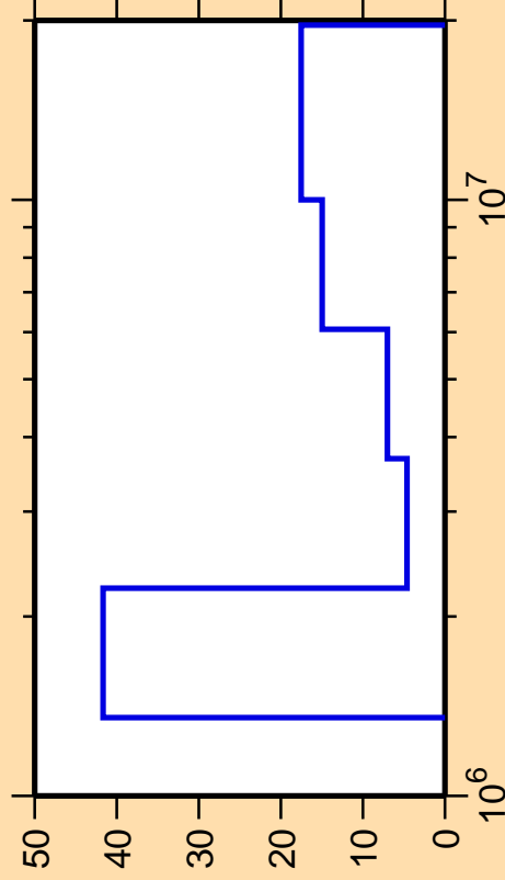
\Delta\sigma/\sigma vs. E for ^{138}\text{Cs}(n, ncont.)
