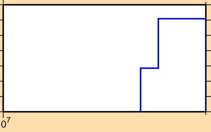
\sigma vs. E for ^{139}\text{Cs}(n,p\alpha)
