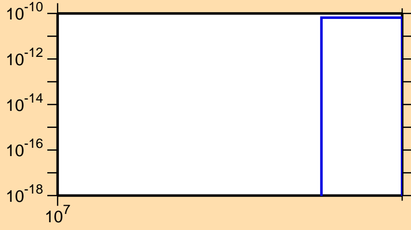
\sigma vs. E for ^{139}\text{Cs} (mt 11)
