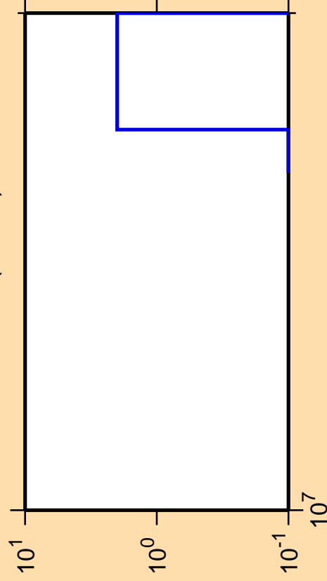
\Delta\sigma/\sigma vs. E for ^{139}\text{Cs} (mt 45)
