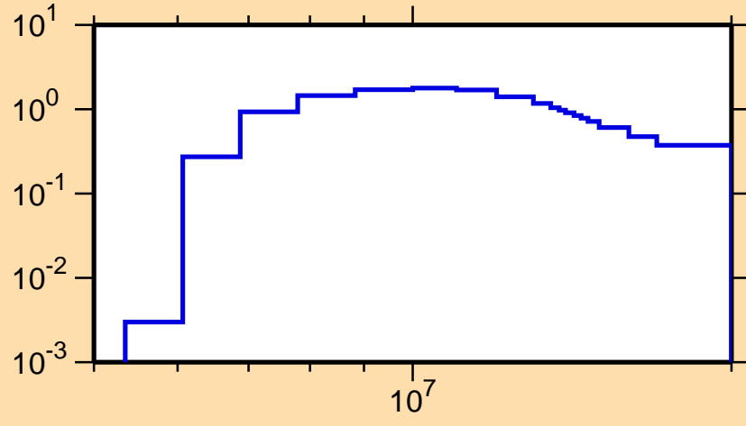
\sigma vs. E for ^{139}\text{Cs}(n,2n)
