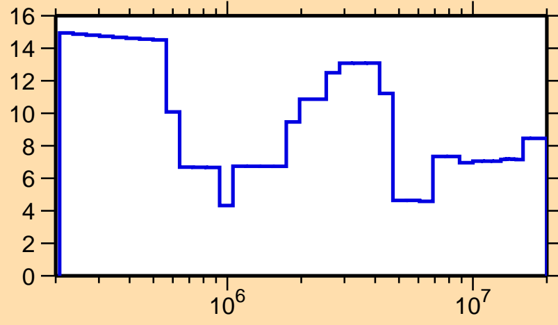
\Delta\sigma/\sigma vs. E for ^{139}\text{Cs}(n,\text{el.})
