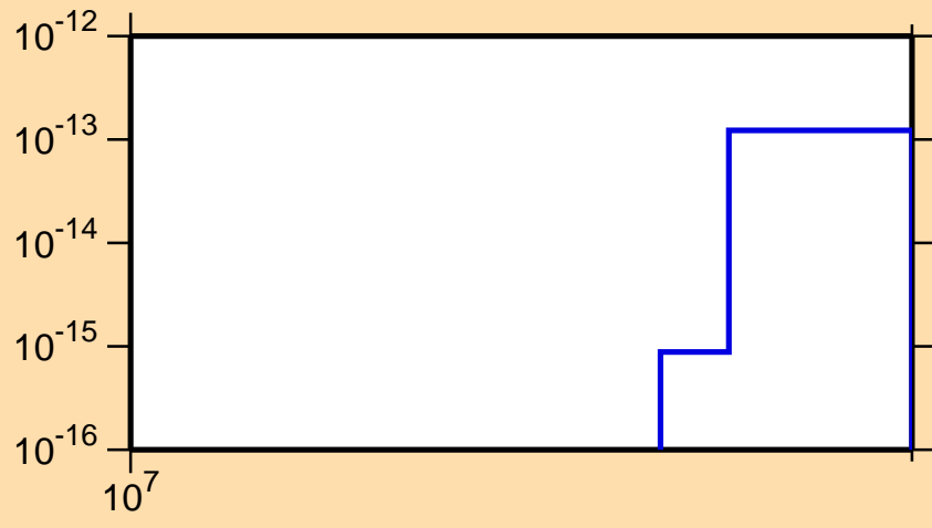
\sigma vs. E for ^{139}\text{Cs}(n,3n\alpha)
