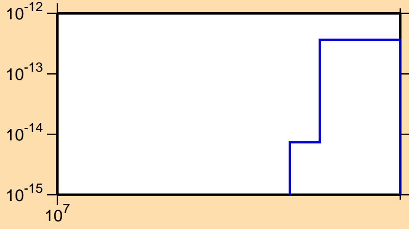
\sigma vs. E for ^{139}\text{Cs} (mt 45)
