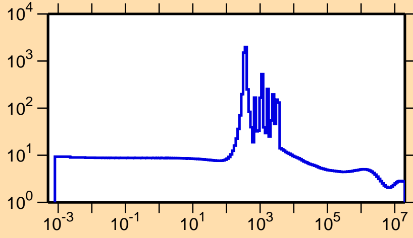
\sigma vs. E for ^{139}\text{Cs}(n,\text{el.})
