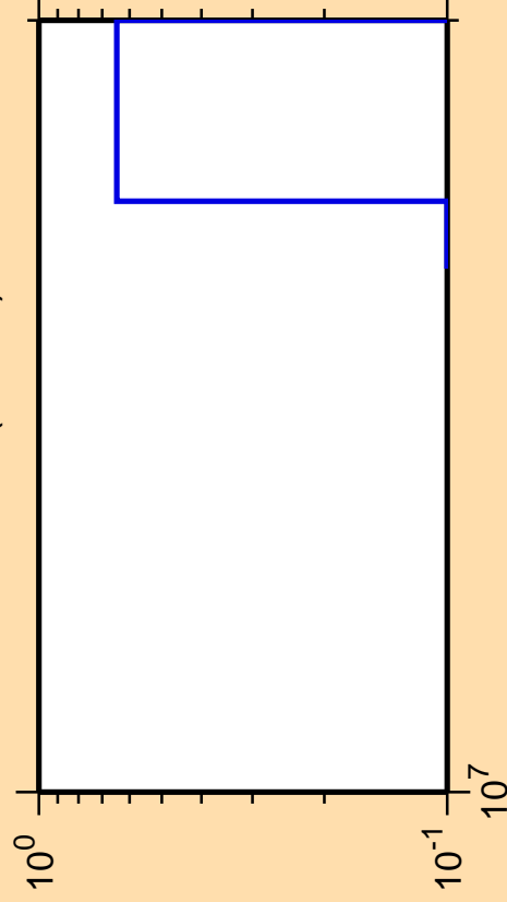
\Delta\sigma/\sigma vs. E for ^{139}\text{Cs}(n,3n\alpha)
