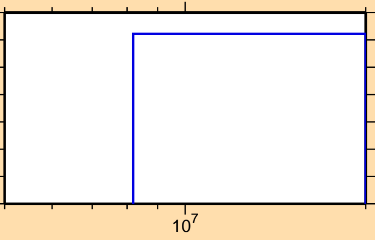
\sigma vs. E for ^{139}\text{Cs}(n,2np)
