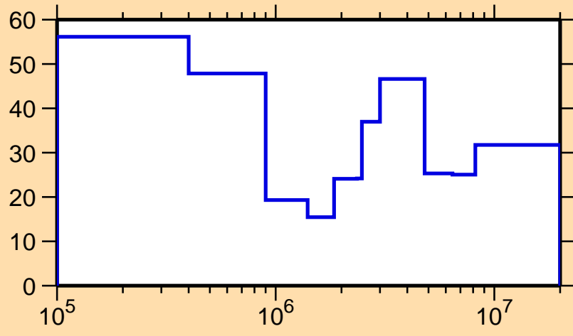
\Delta\sigma/\sigma vs. E for ^{139}\text{Cs}(n,n_1)
