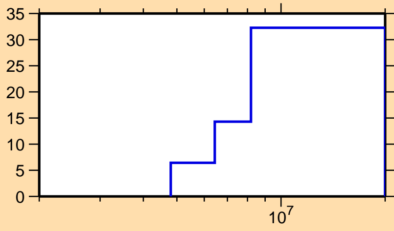
\Delta\sigma/\sigma vs. E for ^{139}\text{Cs}(n,n\text{cont.})
