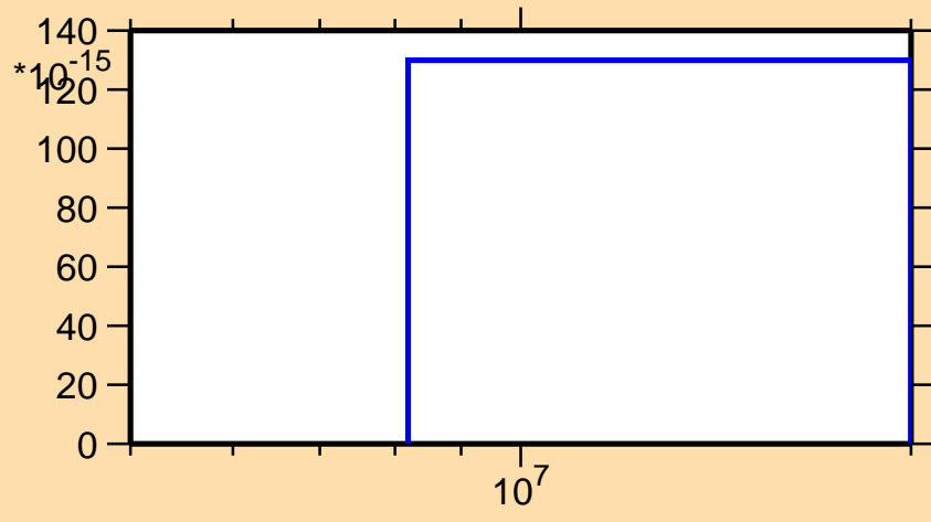
\sigma vs. E for ^{139}\text{Cs}(\text{mt117})
