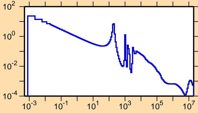
\sigma vs. E for ^{140}\text{Cs}(n,\gamma)
