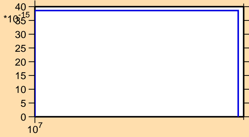
\sigma vs. E for ^{140}\text{Cs}(\text{mt117})
