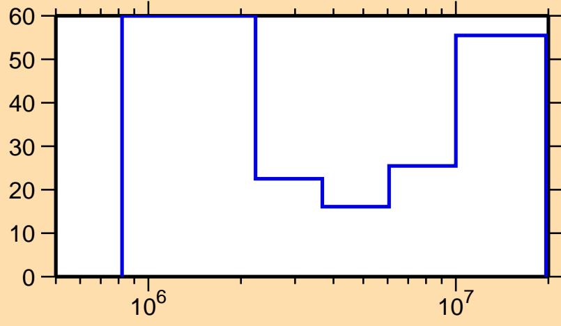
\Delta\sigma/\sigma vs. E for ^{140}\text{Cs}(n,n\text{cont.})
