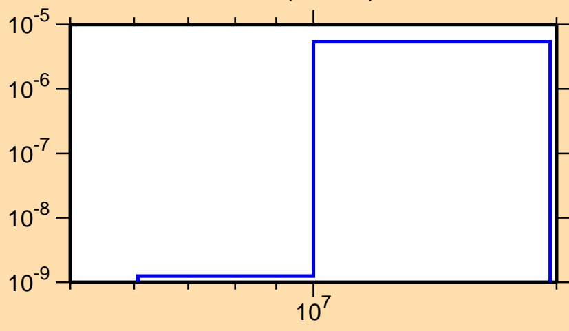
\sigma vs. E for ^{140}\text{Cs}(n,2n\alpha)
