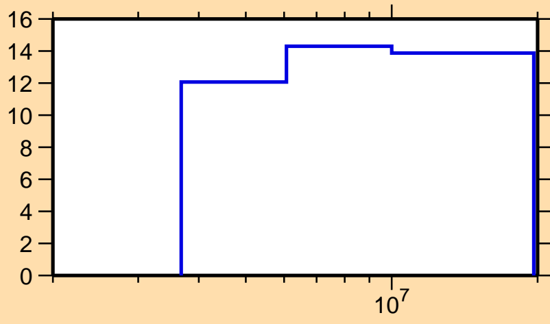
\Delta\sigma/\sigma vs. E for ^{140}\text{Cs}(n,\text{tot.})
