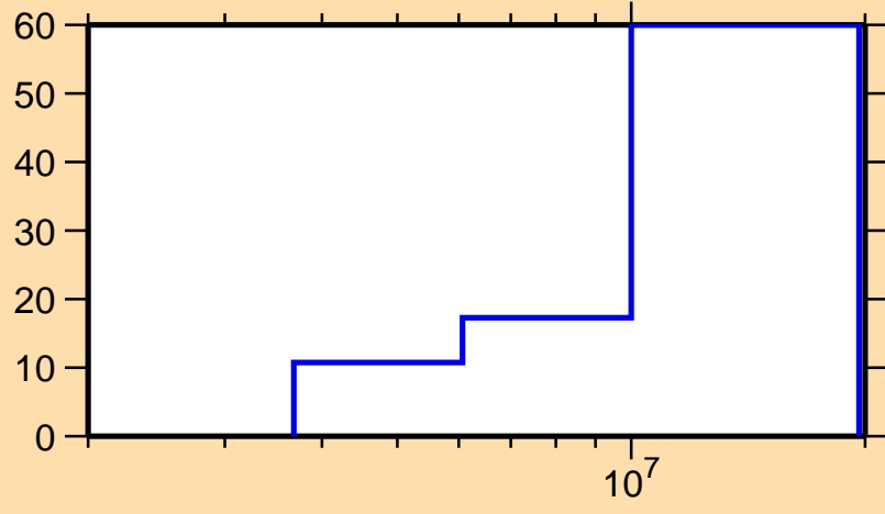
\Delta\sigma/\sigma vs. E for ^{140}\text{Cs}(n,2n)
