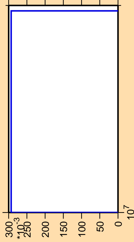
\Delta\sigma/\sigma vs. E for ^{140}\text{Cs}(\text{mt117})
