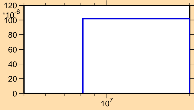
\sigma vs. E for ^{140}\text{Cs}(n,np)
