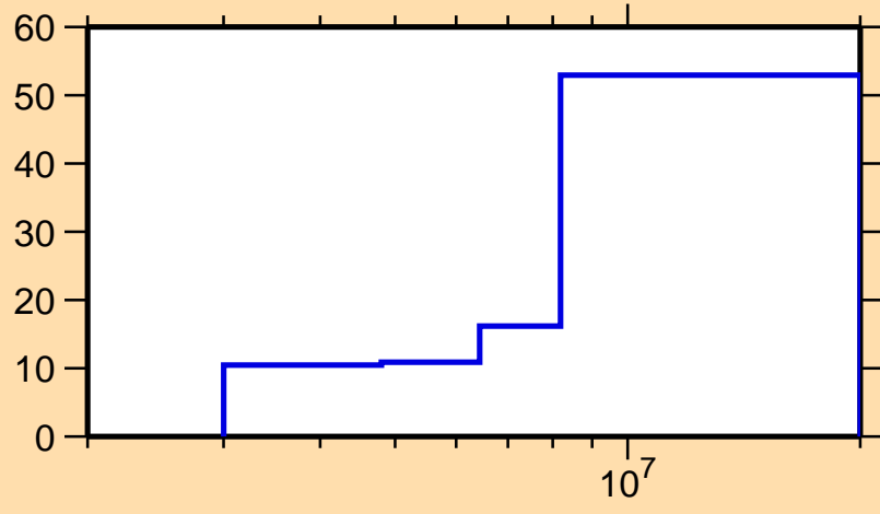
\Delta\sigma/\sigma vs. E for ^{140}\text{Cs}(n,2n)
