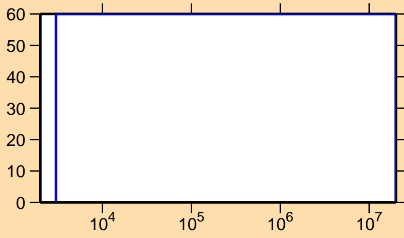
\Delta\sigma/\sigma vs. E for ^{140}\text{Cs}(n,\gamma)
