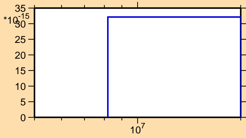
\sigma vs. E for ^{140}\text{Cs}(\text{mt117})
