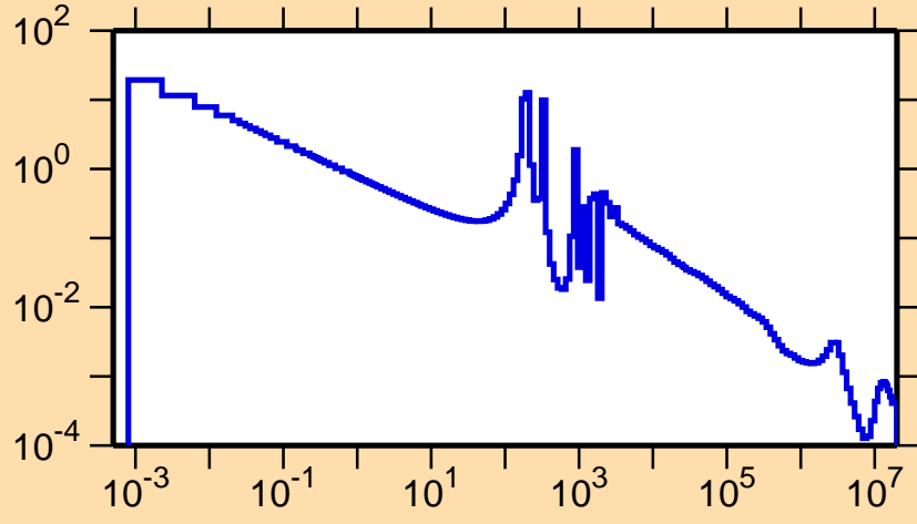
\sigma vs. E for ^{141}\text{Cs}(n,\gamma)
