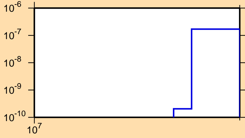
\sigma vs. E for ^{141}\text{Cs}(n,2np)
