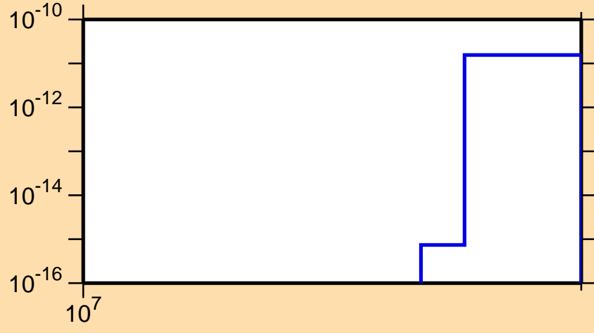
\sigma vs. E for ^{141}\text{Cs} (mt 11)
