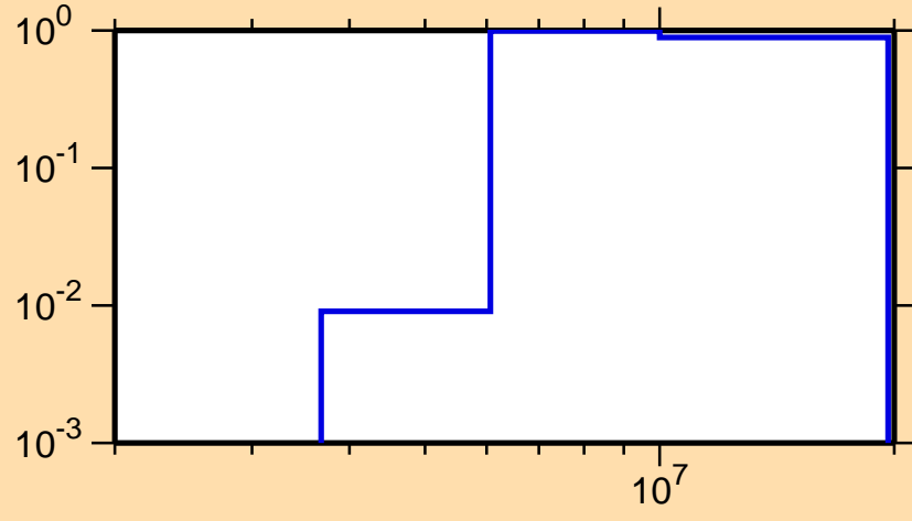
\sigma vs. E for ^{141}\text{Cs}(n,2n)
