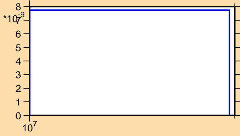
\sigma vs. E for ^{141}\text{Cs}(n,3n\alpha)
