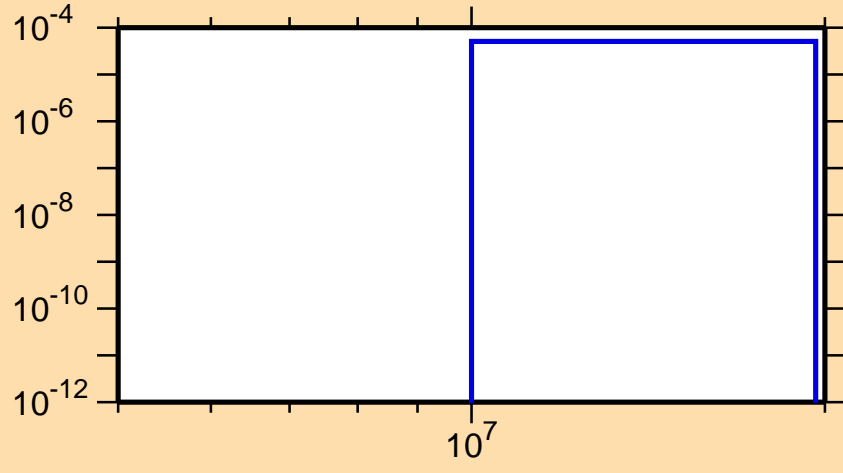
\sigma vs. E for ^{141}\text{Cs}(n,np)
