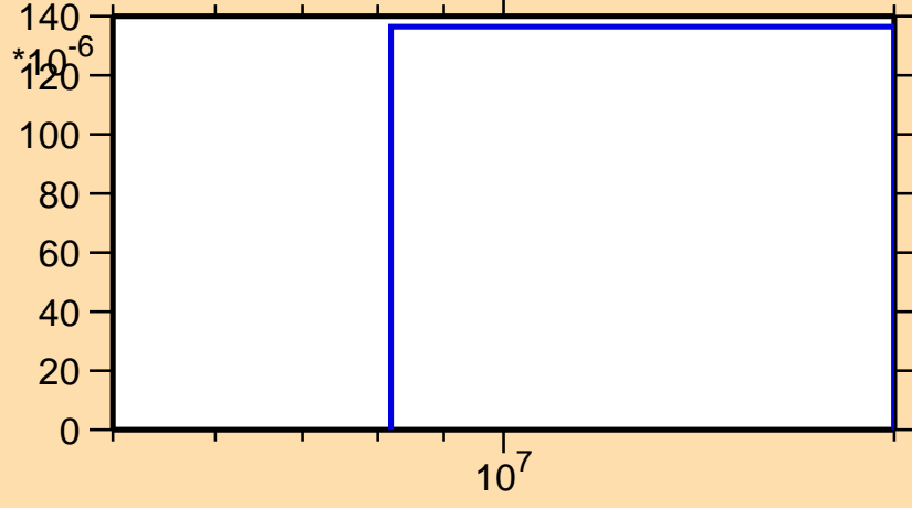
\sigma vs. E for ^{141}\text{Cs}(n,d)
