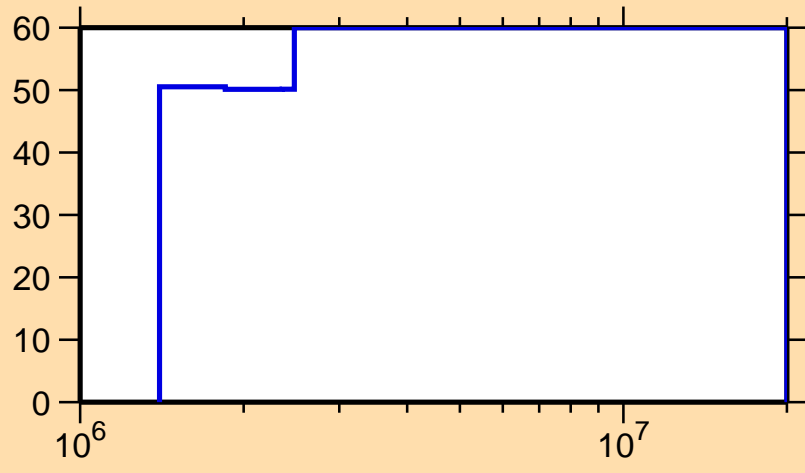
\Delta\sigma/\sigma vs. E for ^{141}\text{Cs}(n,\gamma)
