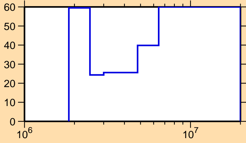
\Delta\sigma/\sigma vs. E for ^{141}\text{Cs}(n,n\text{cont.})
