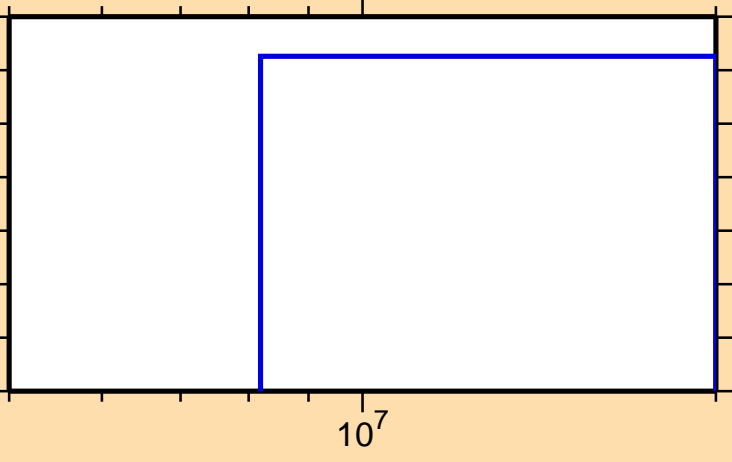
\sigma vs. E for ^{141}\text{Cs}(n,3n\alpha)
