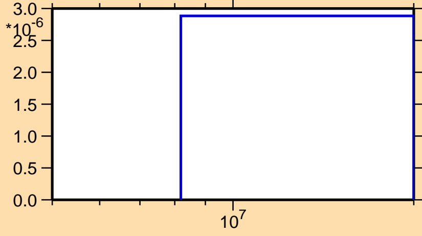
\sigma vs. E for ^{141}\text{Cs}(n,nt)
