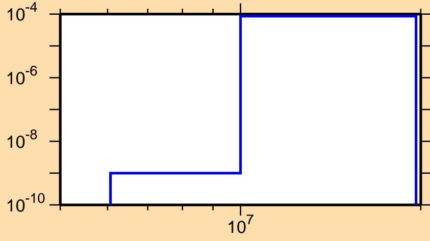
\sigma vs. E for ^{142}\text{Cs}(n,n\alpha)
