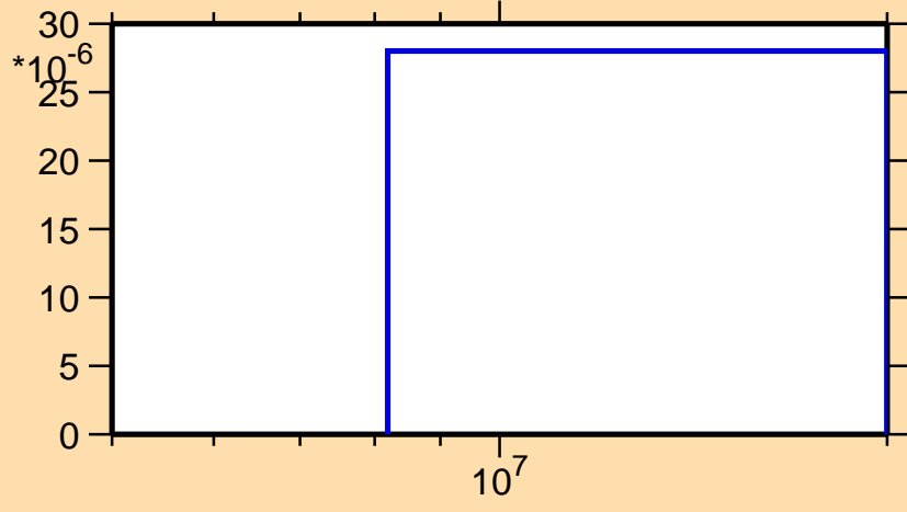
\sigma vs. E for ^{142}\text{Cs}(n,np)
