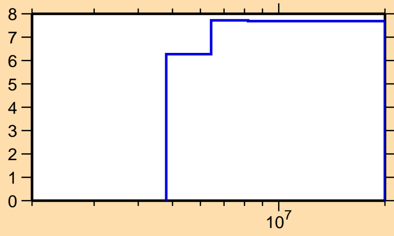
\Delta\sigma/\sigma vs. E for ^{142}\text{Cs}(n,\text{nonel.})
