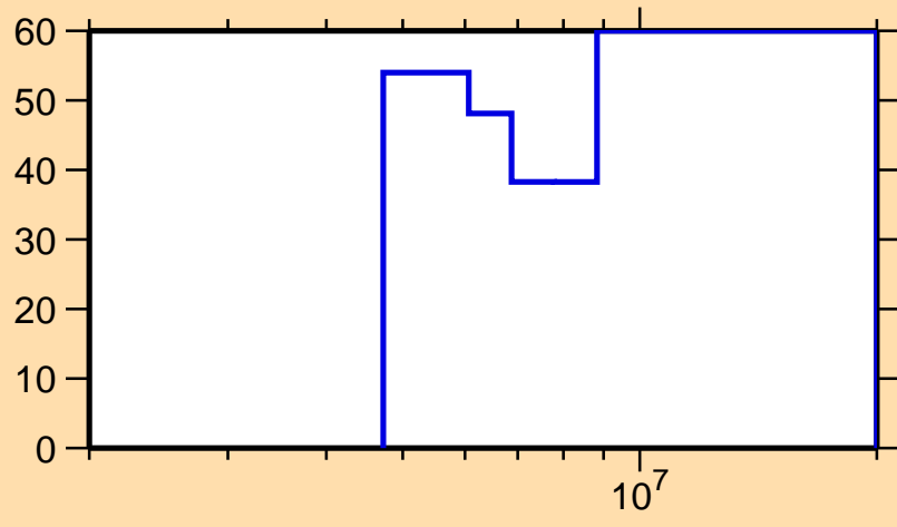
\Delta\sigma/\sigma vs. E for ^{143}\text{Cs}(n,2n)
