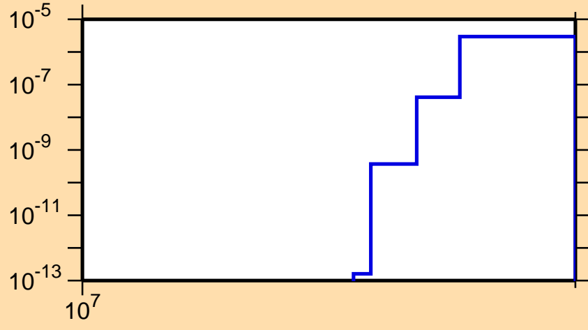
\sigma vs. E for ^{143}\text{Cs}(n,nd)
