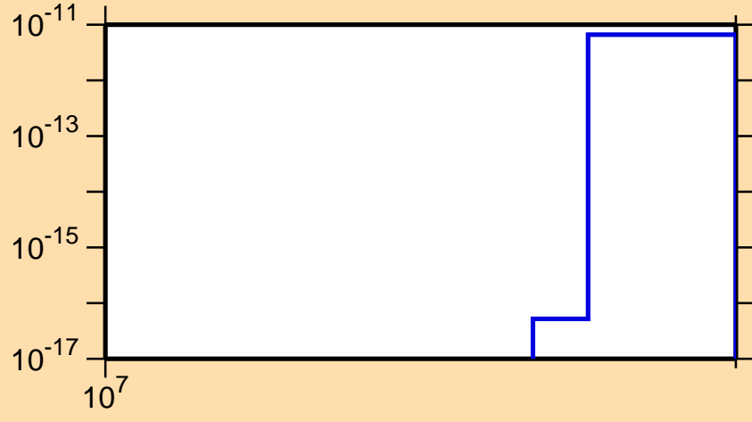
\sigma vs. E for ^{143}\text{Cs} (mt 11)
