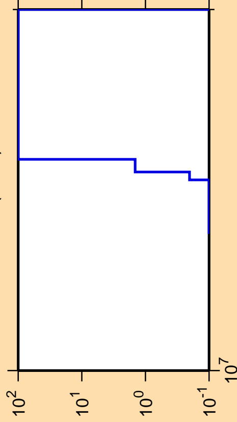
\Delta\sigma/\sigma vs. E for ^{143}\text{Cs}(n,nd)
