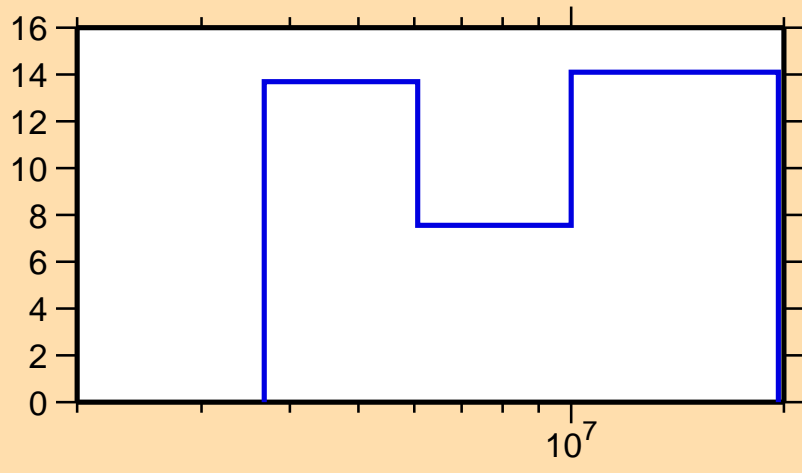
Δσ/σ vs. E for ^{143}\text{Cs}(n,\text{tot.})
