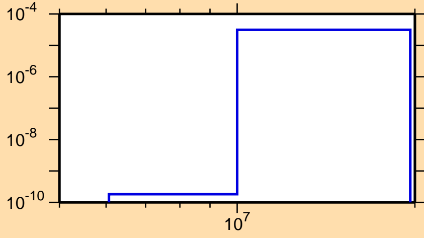
\sigma vs. E for ^{143}\text{Cs}(n,n\alpha)
