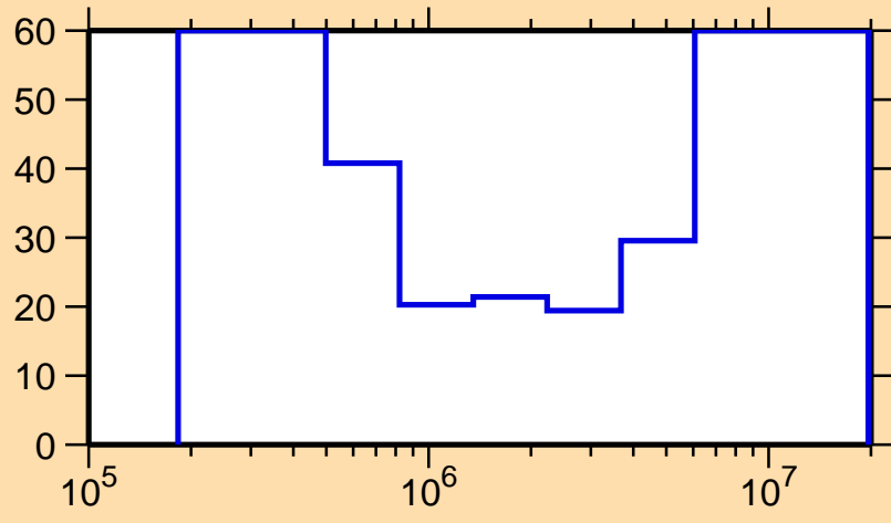
\Delta\sigma/\sigma vs. E for ^{144}\text{Cs}(n,n\text{cont.})
