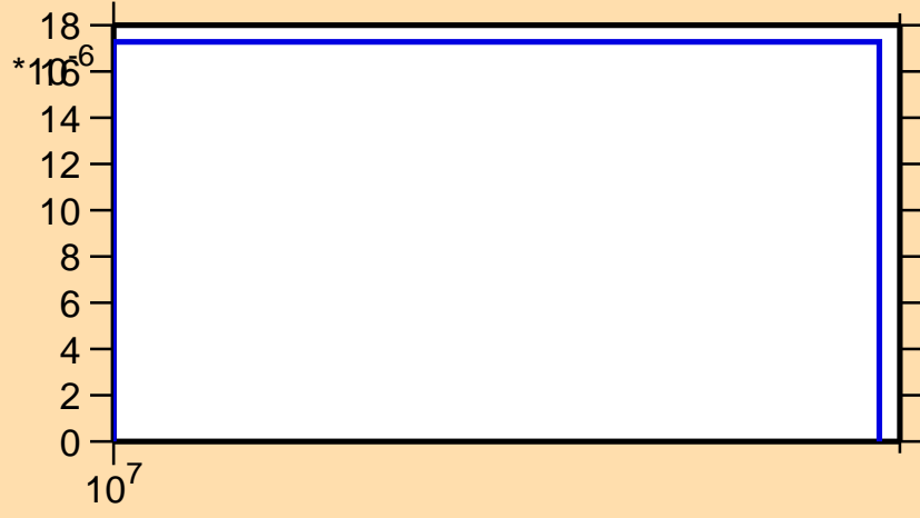
\sigma vs. E for ^{144}\text{Cs}(n,np)
