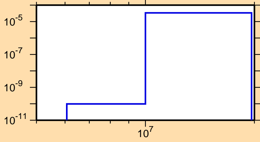
\sigma vs. E for ^{144}\text{Cs}(n,n\alpha)
