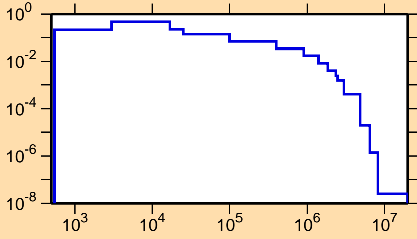
\sigma vs. E for ^{144}\text{Cs}(n,n_1)
