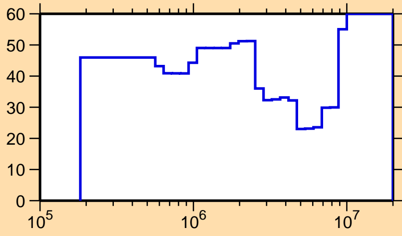
\Delta\sigma/\sigma vs. E for ^{58}\text{Cu}(n,n_1)
