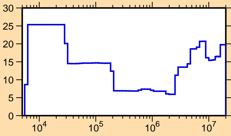
\Delta\sigma/\sigma vs. E for ^{58}\text{Cu}(n,p)
