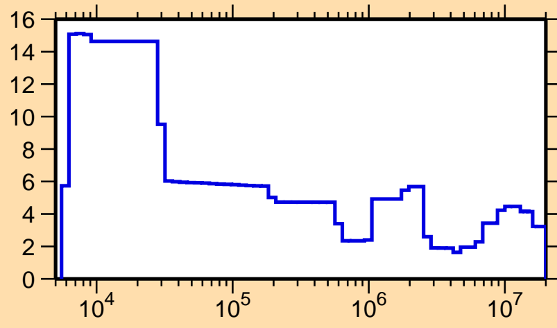
\Delta\sigma/\sigma vs. E for ^{58}\text{Cu}(n,\text{tot.})
