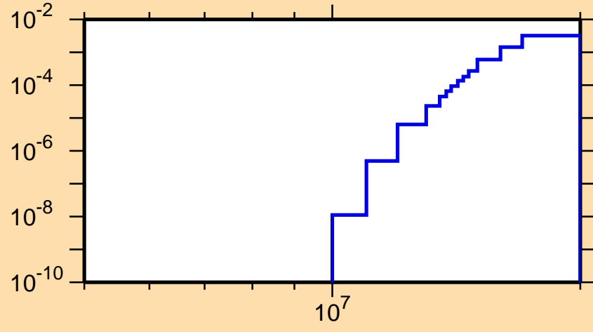
\sigma vs. E for ^{58}\text{Cu}(n,n\alpha)
