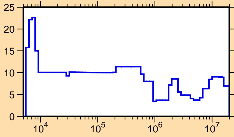
\Delta\sigma/\sigma vs. E for ^{58}\text{Cu}(n,el.)
